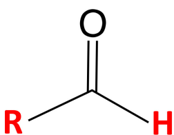
Aldehyde
