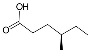
4-methylhexanoic acid
