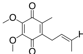
Ubiquinone
