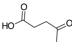
Levulinic acid
