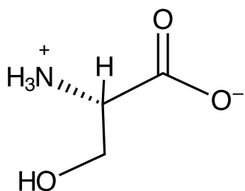
SERINE
