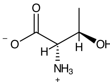
THREONINE
