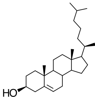
Cholesterol
