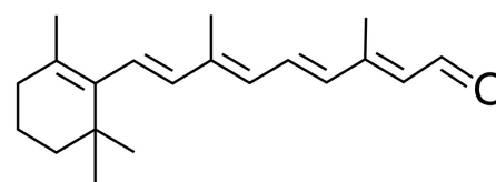
Trans-retinal
