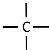
ALKANE
