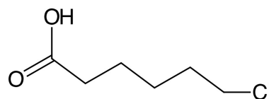
6-chlorohexanoic acid
